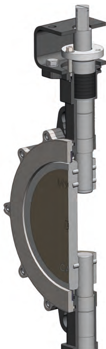
Graphite stem stuffing box
